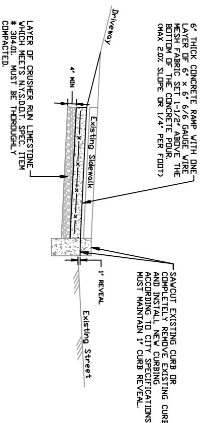
CROSS SECTION
