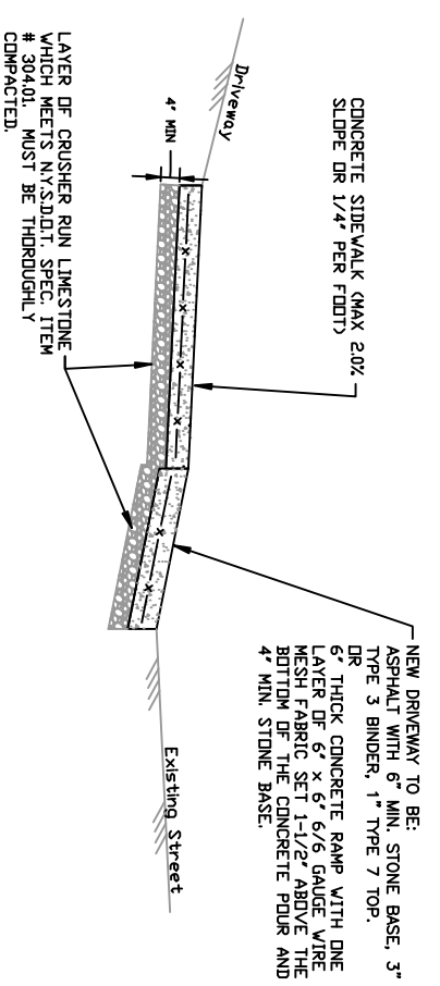
CROSS SECTION
