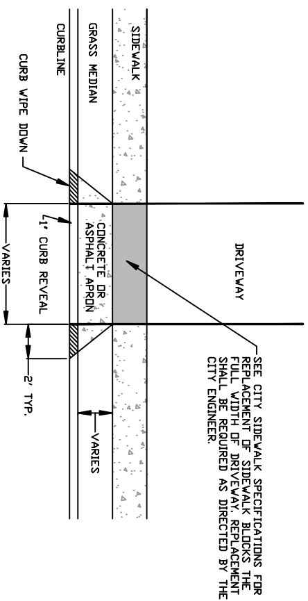
PLAN VIEW
